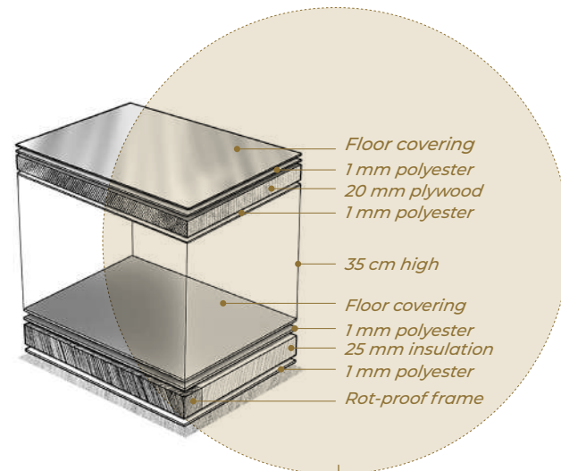
Diagram of the double floor
